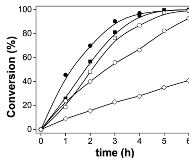
Fig. 5 Conversion of palmitic acid over the catalysts: (■) S-100, (●) S-200, (□) S-300, (○) S-400 and (◇) non-sulfide reference.
