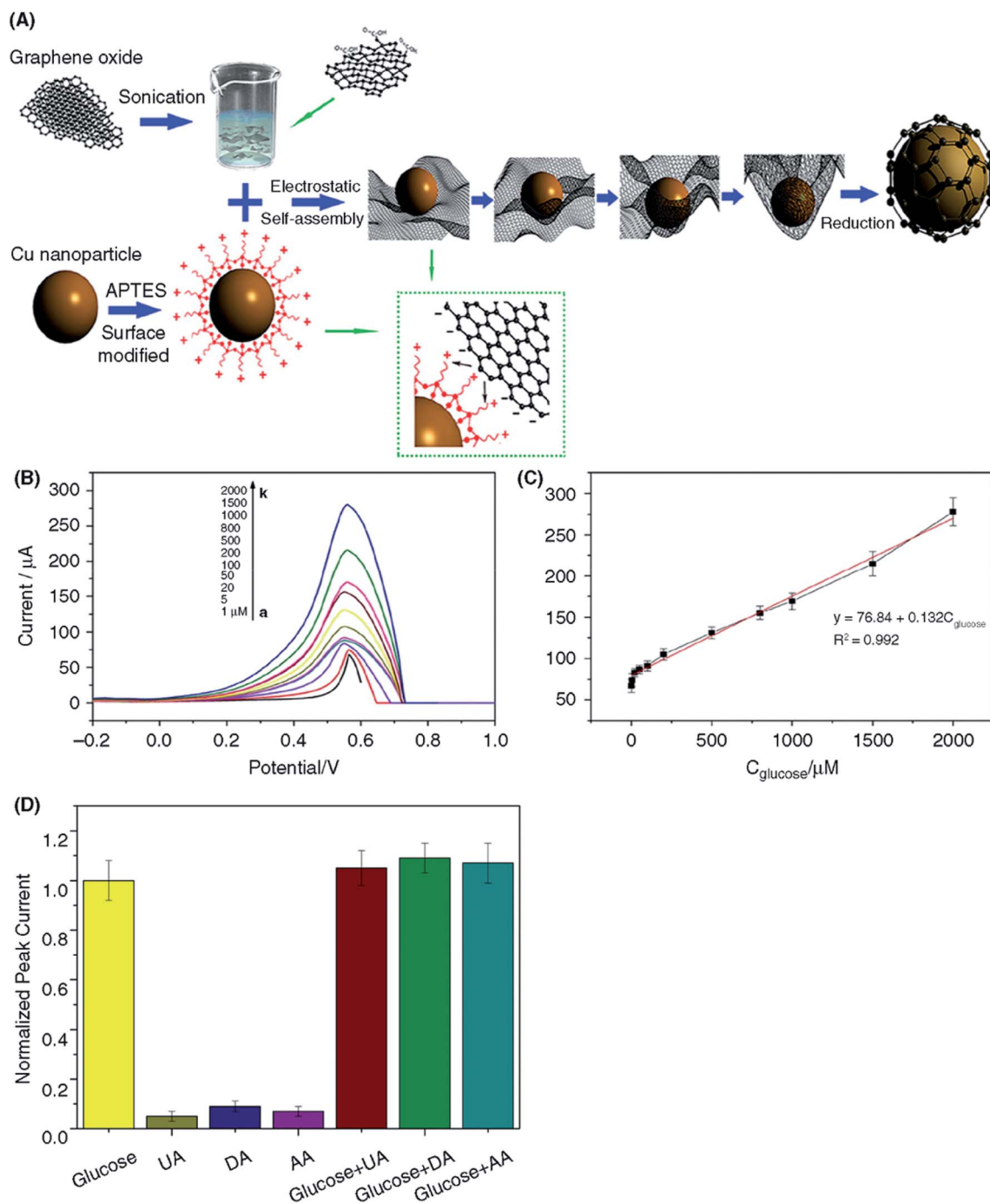
Fig. 10 (A) Schematic illustration of the preparation of graphene-encapsulated CuNPs. (B) DPV responses of graphene-encapsulated CuNPs composites at different concentrations (from a to k: 1– 2000 \mu\text{M} ) of glucose in 0.1 M NaOH. (C) Linear relationship between the peak current and the glucose concentration. (D) Normalized DPV peak current of the CuNPs@rGO composites with the addition of 1.0 mM glucose as the control and in the presence of 2.0 mM uric acid (UA), 2.0 mM dopamine (DA), and 2.0 mM ascorbic acid (AA) as interferents and their corresponding mixtures. The CuNPs@rGO composite-based sensor shows high selectivity for detecting glucose. [Reprinted with permission from ref. 279, Q. Zhang, Q. Luo, Z. Qin, L. Liu, Z. Wu, B. Shen and W. Hu, Self-Assembly of Graphene-Encapsulated Cu Composites for Nonenzymatic Glucose Sensing, ACS Omega , 2018, 3, 3420–3428. Copyright© American Chemical Society.]
