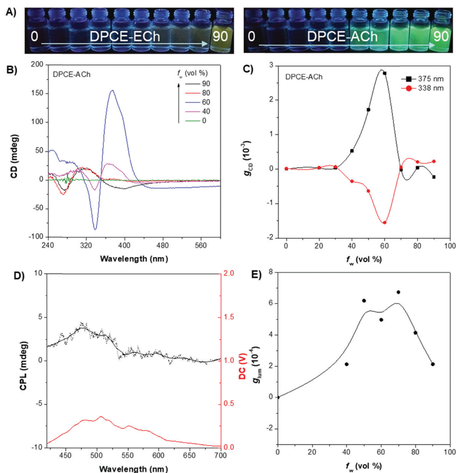
Fig. 2 (A) Fluorescence photographs of DPCE-ECh and DPCE-ACh in THF/H 2 O mixtures with different water fractions ( f_w ). (B) CD spectra and corresponding (C) g_{\text{abs}} factor of DPCE-ACh in THF/H 2 O mixtures with different f_w . (D) CPL spectra of DPCE-ACh in THF/H 2 O mixtures at f_w = 60\% . (E) g_{\text{lum}} factor of DPCE-ACh in THF/H 2 O mixtures with f_w from 40% to 90%. Solution concentration: 5 \times 10^{-5} M.
