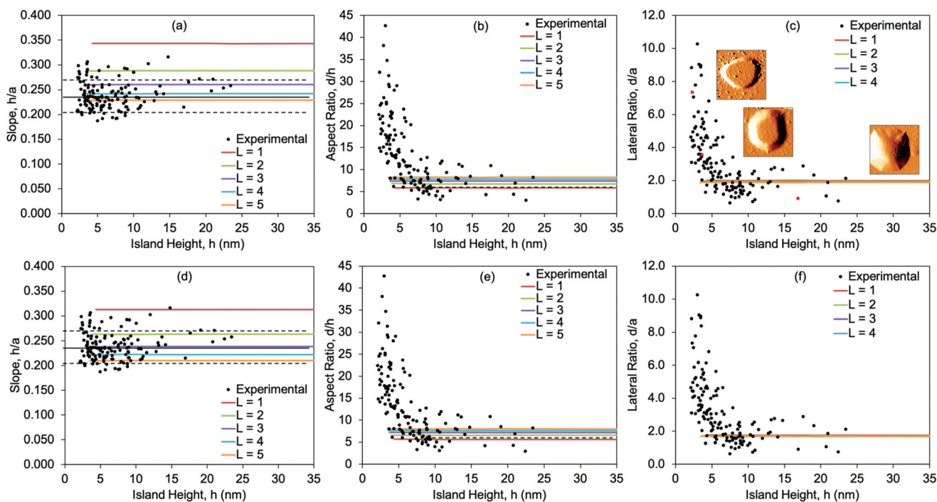
Fig. 3 Experimental and theoretical dimension ratios h/a , d/h , and d/a , vs. h . Theoretical results are shown by colored lines for 1 \leq L \leq 5 . Panels (a, b, c) give results for the free SLBT model, and (d, e, f) for the clamped SLBT model. In panels (a, d) the experimental average is the solid horizontal black line at h/a = 0.24 , and the limits of \pm 1\sigma (the standard error) are shown by the dashed horizontal black lines. In panels (b, e) the experimental average of d/h = 7.3 for h > 10 nm is shown by the dashed horizontal black line. Panel (c) also shows STM images of islands to illustrate the difference in d/a . Red data points correspond to STM image insets. The STM image sizes in panel (c), from highest d/a to lowest d/a , are: 105 \times 105 \text{ nm}^2 ; 80 \times 80 \text{ nm}^2 ; 250 \times 250 \text{ nm}^2 .
