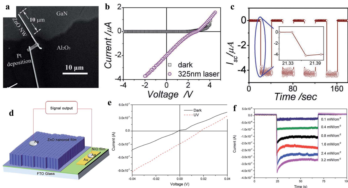
Fig. 12 ZnO/GaN junction self-powered PD: (a and b) SEM image of n-ZnO NW/p-GaN junction and the respective I-V profiles under dark and UV illumination conditions, respectively. (c) Cyclic short circuit current–time response of the PD in the absence of a bias voltage with a 325 nm laser turned on and off repeatedly. Reproduced with permission from ref. 190 Copyright 2011 WILEY-VCH. p-NiO/n-ZnO NRs junction: (d and e) device schematic and I-V profiles before and after exposure to UV light. (f) Variation in current with respect to UV illumination intensity at zero bias condition. Reproduced with permission from ref. 191 Copyright 2015 Royal Society of Chemistry.
