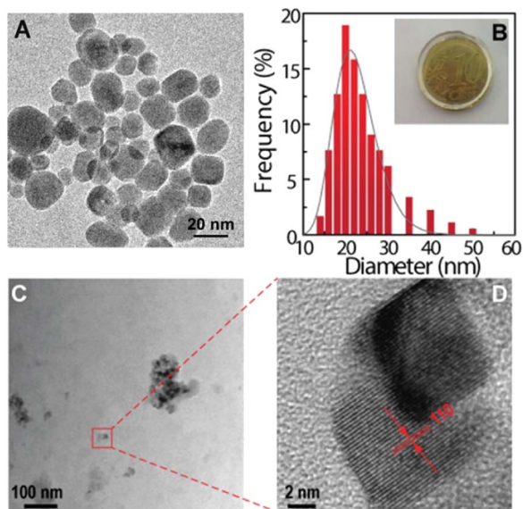
Fig. 1 (A) HRTEM image of the \text{NaYF}_4:\text{Yb}^{3+}/\text{Er}^{3+} UCNP. (B) Particle size distribution obtained from analysis of the HRTEM images. The solid line is the best fit to a log-normal distribution with a diameter of 23 \pm 5 nm. The inset shows a digital photograph of the HyTa- \text{Yb}^{3+}/\text{Er}^{3+} hybrid. (C and D) HRTEM images of the HyTa- \text{Yb}^{3+}/\text{Er}^{3+} hybrid at different magnifications. The interplanar distance marked corresponds to 0.30 nm.
