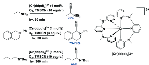
Fig. 44 \alpha -Aminonitrile formation using [\text{Cr}(\text{dddpd})_2]^{3+} , as the PC.
