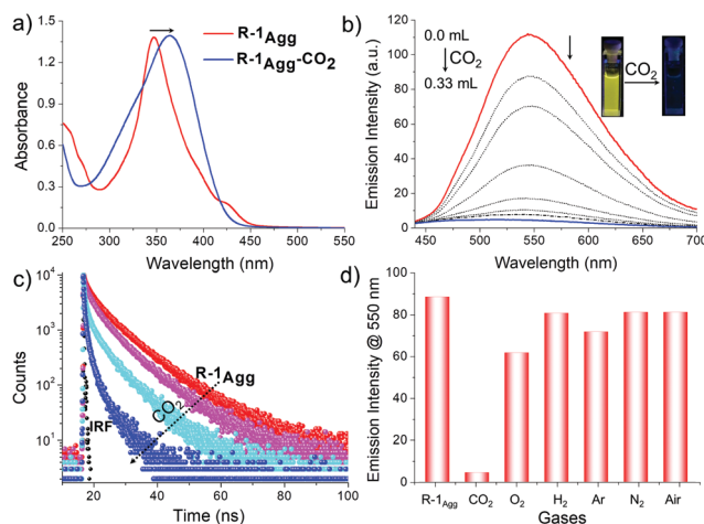
Fig. 2 (a) Absorption spectra of R-1 ( 1 \times 10^{-4} M) in aqueous medium (water/DMSO, 99/1 v/v) after purging with excess amount of CO 2 (0.33 mL). (b) Emission spectra of R-1 ( 1 \times 10^{-4} M, \lambda_{ex} = 370 nm) in the presence of different concentrations of CO 2 (0, 0.016, 0.032, 0.048, 0.064, 0.080, 0.096, and 0.33 mL). Inset shows the fluorescence change of R-1 under UV illumination ( \lambda_{ex} = 365 nm) before and after purging with CO 2 . (c) Fluorescence lifetime decay profile of R-1 ( \lambda_{ex} = 370 nm, \lambda_{em} = 550 nm) in the presence of increasing CO 2 concentrations (0, 0.016, 0.048 and 0.33 mL). IRF = instrument response function. (d) Fluorescence response ( \lambda_{ex} = 370 nm) of R-1 towards CO 2 after purging with different gases (3.0 mL) in aqueous medium; from left to right: R-1 , CO 2 , O 2 , H 2 , Ar, N 2 and air.
