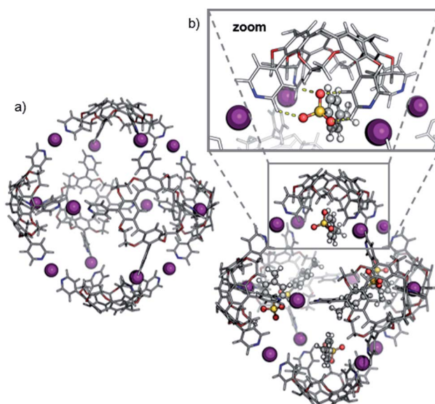
Fig. 4 Geometry-optimized structure of the hexameric halogen-bonded capsule 2 (a) in the absence of tosylate ions ( [6 \cdot \text{C}_6\text{H}_5 + 12\text{I}]^{12+} ) and (b) with six tosylate anions ( [6 \cdot \text{C}_6\text{H}_5 + 12\text{I} + 6 \cdot \text{OTs}]^{6+} ). The n -hexyl chains are omitted for clarity. Inset: binding situation of a tosylate counterion.
