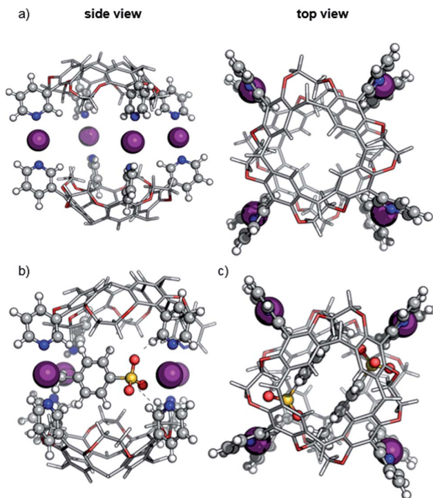
Fig. 2 Geometry-optimized structures of dimeric halogen-bonded capsule 1 (a) in the absence of tosylate counterions ( [2 \cdot \text{C}_\text{D} + 4\text{I}]^{4+} ; side and top view); (b) with one tosylate inside the cavity ( [2 \cdot \text{C}_\text{D} + 4\text{I} + \text{OTs}]^{3+} , [\text{C}_{\text{aryl}}-\text{H} \cdots \text{O}^-] interactions are marked with dotted lines); (c) with two tosylates inside the cavity ( [2 \cdot \text{C}_\text{D} + 4\text{I} + 2\text{OTs}]^{2+} ). PBE0/def2-SVP was used for \text{I}^+ , pyridines and tosylates (ball-and-stick representation); AM1 for the cavitand scaffold (stick representation). For clarity, the n -hexyl chains are omitted in the images.
