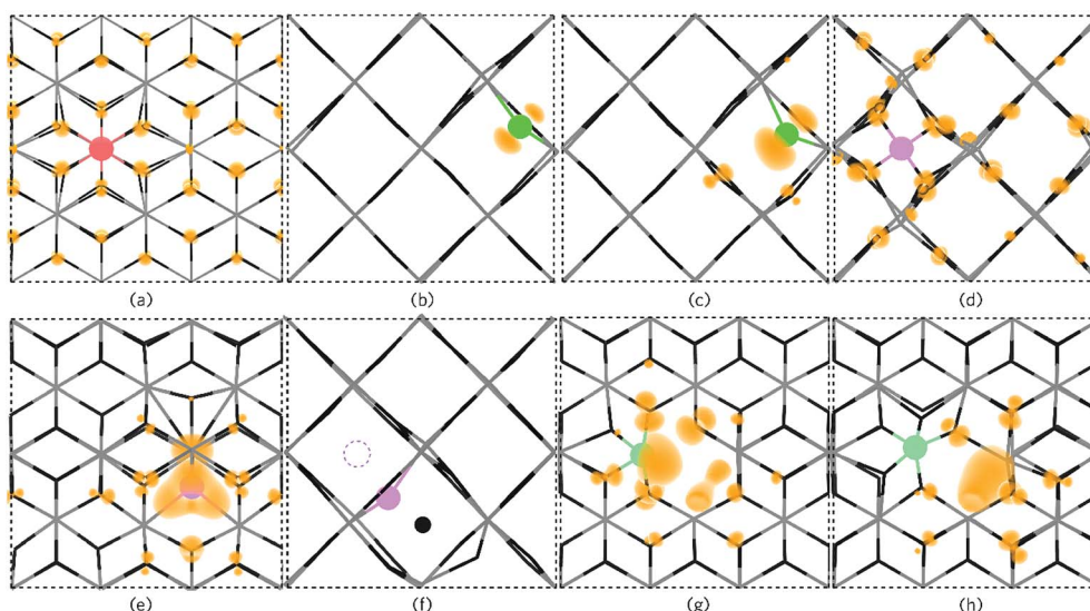
Fig. 7 The partial electron charge densities (orange) for (a) P_{Sn} viewed along \{010\} with a charge density of 0.002 \text{ eV } \text{Å}^{-1} , (b) P_O^0 and (c) P_O^{1-} as viewed along the \{001\} direction with a charge density of 0.02 \text{ eV } \text{Å}^{-1} . P_i^{3+} is depicted in (d) along the \{001\} direction with a charge density of 0.008 \text{ eV } \text{Å}^{-1} and P_i^{3-} is shown in (e) along \{010\} with a charge density of 0.02 \text{ eV } \text{Å}^{-1} where a large triple polaron is seen. In (f), P_i^{3-} is viewed along the \{001\} axis presenting the displacement of a lattice O to an interstitial site by P (the original interstitial position is shown by the dashed circle). (g) and (h) displays the defect cluster [P_{Sn} + V_O] in both the neutral and 1+ charge states respectively as viewed along \{010\} and plotted from 0-0.01 \text{ eV } \text{Å}^{-1} . In each panel the \text{SnO}_2 is depicted by the grey (Sn) and black (O) wire frame model with the P species colour coded to Fig. 6.
