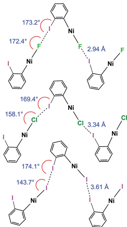
Scheme 6 Halogen bond length and \text{C-I}\cdots\text{Ni} and \text{I}\cdots\text{X}\text{-Ni} angles for 1oF , 1oCl and 1oI ( \alpha ) (phosphines and aromatic fluorines omitted, for esd's see Table 2).
