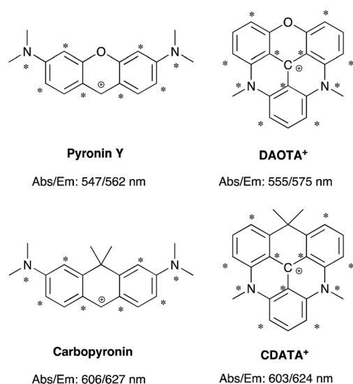
Chart 2 Chromophore analysis of Pyronin Y, carbopyronin, DAOTA + , and CDAOTA + . The values of the lowest energy absorption maximum (Abs) and emission maximum (Em) are from this work and ref. 7.
