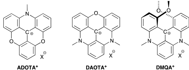
Chart 1 Azadioxatriangulenium (ADOTA + ), diazaoxatriangulenium (DAOTA + ) and dimethoxyquinacridinium (DMQA + ). X - refers to an arbitrary anion.
