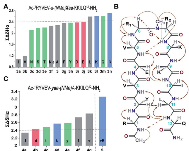
Fig. 4 (A) \sum \text{CSD} of the primary library with L-amino acid substitutions (Xaa) at the i+2 site. (B) The characteristic NOEs, where the thick arrows denote strong (1.8–2.1 Å), the thin arrows denote medium (2.2–2.5 Å) and the broken arrows denote weak (>2.6 Å) NOEs. (C) \sum \text{CSD} of the secondary library with i+1 substitutions (yaa) along with 5 derived from the combination of 4g and 3n. All the NMR measurements were done in acetate buffer (pH 3.8) at 25 °C.
