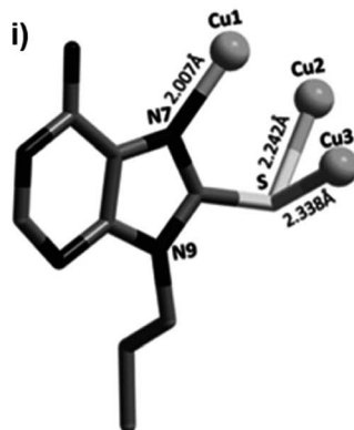
Fig. 26 (a–f) 2D AFM image of time-dependent solution phase growth of copper complex on glass surface. Scale bars: 5 \mu\text{m} ; (g) 3D AFM image of cuboidal aggregate; (h) periodic increase in Z-height over 0 to 30 days; (i) Crystal structure of copper complex 4 (Reproduced with permission from ref. 124 © 2014 WILEY-VCH Verlag GmbH & Co. KGaA, Weinheim).
