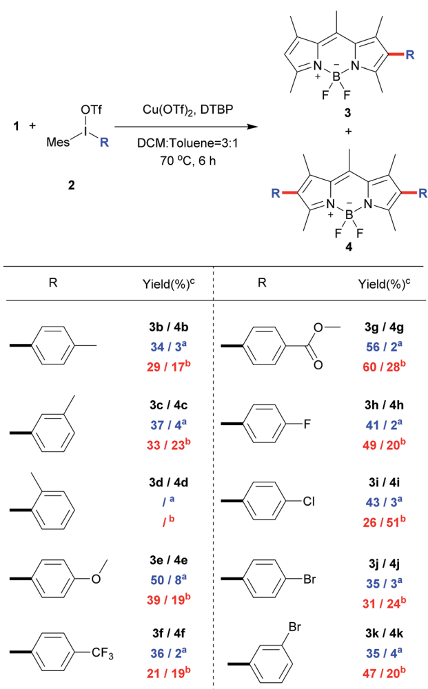
Scheme 3 Direct C–H arylation of BODIPY 1 with different diaryliodonium triflates. a Condition A: 0.8 equiv. of 2 was used; b condition B: 2.4 equiv. of 2 was used; c isolated yield.
