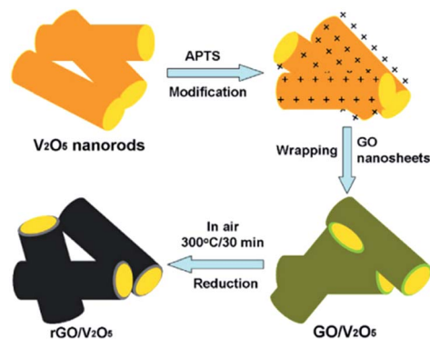
Fig. 14 Schematic of the fabrication of rGO wrapped V_2O_5 nanorods. 140
