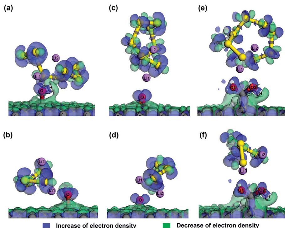
Fig. 6 Deformation charge density at \text{Li}_2\text{S}_8 and \text{Li}_2\text{S}_4 adsorption sites of (a and b) hG, (c and d) eG and (e and f) cG. (The increase/decrease of electron density is denoted by blue/green, respectively.)
