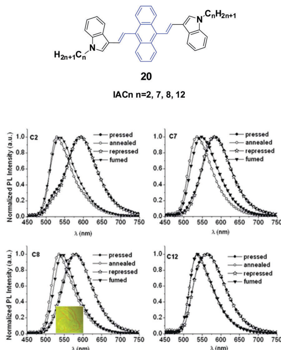
Fig. 7 (Top) The molecular structure of compound 20. (Bottom) Normalized emission spectra of IAC n samples upon external stimuli (excited at 470 nm). Inset: A piece of filter paper soaked with IAC8 on which a rabbit is drawn using a metal spatula and illuminated under UV light. Reproduced with permission from ref. 43. Copyright 2015 The Royal Society of Chemistry.
