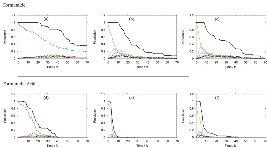
Fig. 2 Diabatic state populations from DD-vMCG simulations of formamide (top) and formimic acid (bottom) starting with a vertical excitation to various states: (a and d) S_1 , (b and e) S_2 and (c and f) S_3 . Key: S_0 : purple; S_1 : green; S_2 : light blue; S_3 : orange; S_4 : yellow; S_5 : dark blue; S_6 : red; S_7 : black. Total density (norm 2 ): thick black.
