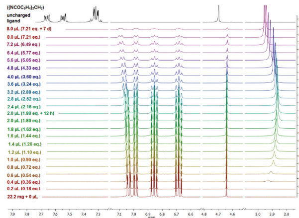
Fig. 4 Stacked ^1\text{H} NMR spectra (thf- d_8 ) of a titration experiment of [\{(\text{NCOC}_6\text{H}_4)_2\text{CH}\}\text{K}(\text{thf})]_n ( 2 ) with water and a free uncharged (\{(\text{NCOC}_6\text{H}_4)_2\text{CH}_2\}) ligand (black).
