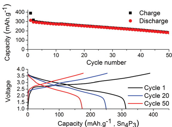
Fig. 5 Galvanostatic cycling of tin phosphide vs. Prussian Blue using electrolyte of 1 M NaPF 6 dissolved in EC : DEC (1 : 1) with 10 vol% FEC. The cell utilized an oversized cathode and capacity is based on the active material in the anode.
