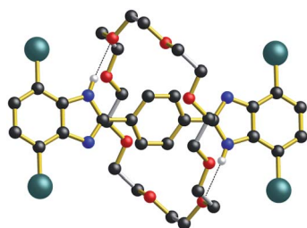
Fig. 7 Ball-and-stick representation of the single-crystal X-ray structure of the [2]rotaxane molecular shuttle \mathbf{R}_1\text{-Br} ( n = 1 ). Only H-atoms involved in hydrogen bonds are shown for clarity. Color key: teal = bromine, red = O; blue = N, black = C; white = H; gold bonds = axle; silver bonds = wheel.
