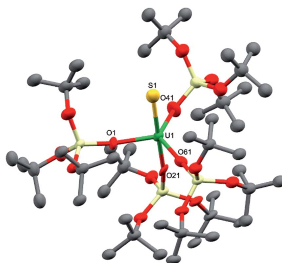
Fig. 5 Molecular structure of the anionic fragment of one of the crystallographically independent pairs of [\text{K}(\text{2.2.2-cryptand})][\text{US}\{\text{OSi}(\text{OTfBu})_3\}_4] in crystals of 8-15tol shown with 50% probability thermal ellipsoids. [\text{K}(\text{2.2.2-cryptand})]^+ , hydrogen atoms and lattice solvent molecules have been omitted for clarity.
