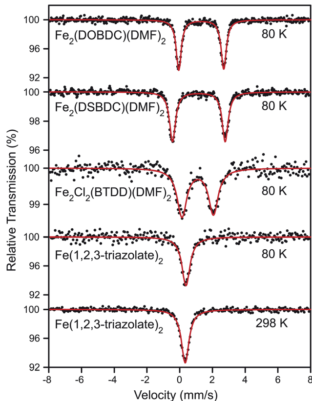
Fig. 4 ^{57}\text{Fe} Mossbauer spectra of \text{Fe}_2(\text{DOBDC})(\text{DMF})_2 , \text{Fe}_2(\text{DSBDC})(\text{DMF})_2 , and \text{Fe}_2\text{Cl}_2(\text{BTDD})(\text{DMF})_2 at 80 K as well as \text{Fe}(\text{1,2,3-triazolate})_2 at 80 and 298 K. All samples were kept in \text{N}_2 atmosphere. Black dots represent experimental data, and red curves represent Lorentzian fitting curves.
