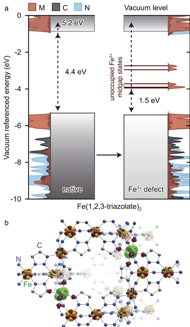
Fig. 8 (a) Calculated energy bands and projected density of states (PDOS) of native \text{Fe}(\text{1,2,3-triazolate})_2 and the hypothetical material \text{Fe}_{1/6}^{\text{III}}\text{Fe}_{5/6}^{\text{II}}(\text{1,2,3-triazolate})_2^{1/6+} . E_{\text{VBM}} are shown on the top and band gaps are shown in the middle of each sub-figure. (b) The spin density of the hypothetical material \text{Fe}_{1/6}^{\text{III}}\text{Fe}_{5/6}^{\text{II}}(\text{1,2,3-triazolate})_2^{1/6+} shows partially delocalized spin across the Fe centers (shown in yellow and red), with some local \text{Fe}^{3+} character emphasized in green.
