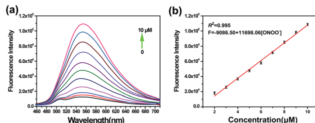
Fig. 2 (a) Fluorescence response of TP-KA (1 \mu\text{M} ) to \text{ONOO}^- (0–10 \mu\text{M} ) in PBS buffer (50 mM, pH 7.4) with 1% DMSO. (b) The linear curve derived from the fluorescence intensity at 560 nm and the \text{ONOO}^- concentration. The spectra were recorded after the incubation of TP-KA with \text{ONOO}^- for 10 min at 37 ^\circ\text{C} . The values are the mean \pm s.d. for n = 3 . \lambda_{\text{ex}}/\lambda_{\text{em}} = 430/560 nm.
