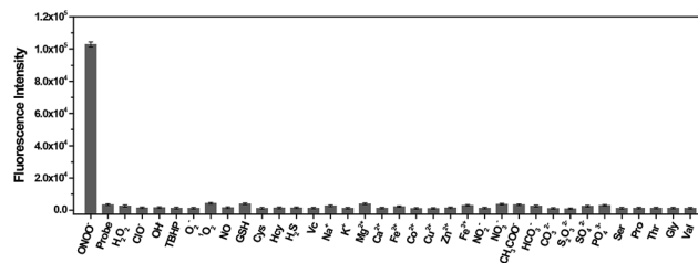
Fig. 1 Fluorescence response of TP-KA (1.0 \mu\text{M} ) with various bio-analytes, including \text{ONOO}^- (10.0 \mu\text{M} ), \text{H}_2\text{O}_2 (200 \mu\text{M} ), other ROS and RNS (10.0 \mu\text{M} ), GSH and Cys (5.0 mM), and other interfering substances (100 mM). The data were recorded after the incubation of TP-KA with various bio-analytes for 10 min at 37 ^\circ\text{C} in PBS buffer (50 mM, 7.4) with 1% DMSO. The values are the mean \pm s.d. for n = 3 . \lambda_{\text{ex}}/\lambda_{\text{em}} = 430/560 nm.
