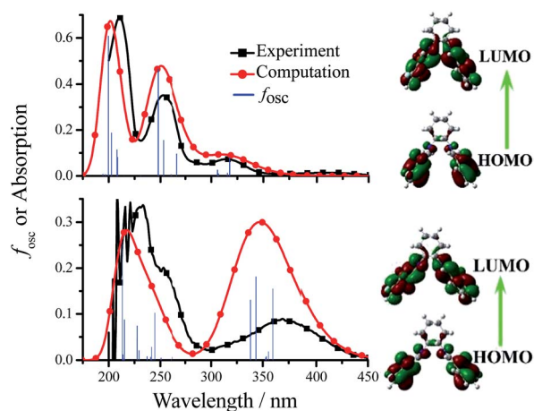
Fig. 12 Computational (gas-phase) and experimental absorption spectra and Frontier molecular orbitals of 3-F-Cy (top, in form of OH) and 3-F-Cy + 100 equivalent of OH ^- (bottom, in form of O ^- ) MeCN solution.
