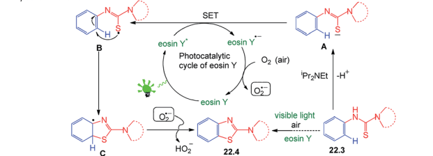
Scheme 22 Aerobic oxidative cyclization of 2-aminobenzothiazole.
