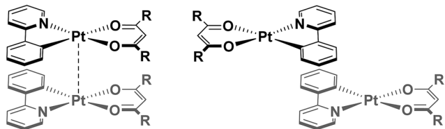
Fig. 1 Pt(II) complexes arranged in a syn -orientation (left) of the ligands showing both \pi – \pi interactions and metal–metal interactions and in an anti -orientation (right) of the ligands with C ^ N \cdots C ^ N \pi – \pi interactions but without further interactions owing to large Pt \cdots Pt and O ^ O \cdots O ^ O ligand distances.
