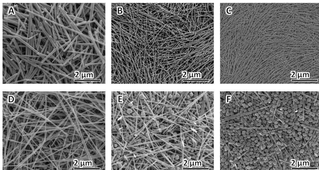
Fig. 4 FE-SEM images of AgNWs synthesized at different [PVP] to [AgNO 3 ] molar ratio: (A) 2 : 1, (B) 4 : 1, (C) 6 : 1, (D) 8 : 1, (E) 10 : 1, and (F) 12 : 1.
