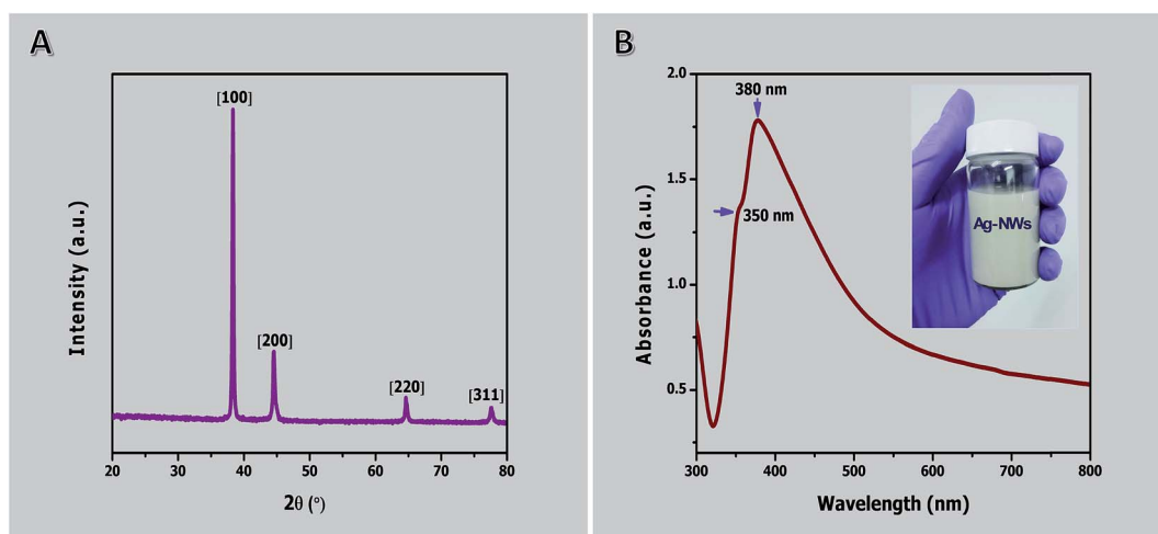
Fig. 5 (A) XRD pattern of the purified as-prepared AgNWs (160 °C; 3 h) indicating FCC crystals. (B) UV-visible absorption spectrum of the purified AgNWs. The inset in (B) shows a photo of AgNW solution, dispersed in ethanol after purification.
