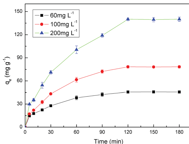
Fig. 7 Effect of contact time on U(VI) adsorption. (Volume, 30 mL; adsorbent dose, 0.03 g; initial concentration, 60, 100 and 200 mg\ L^{-1} ; pH value, 4.0; contact time, 0, 5, 10, 20, 30, 60, 90, 120, 150, 180 min; temperature, 25 °C; rotating speed, 150 rpm.)
