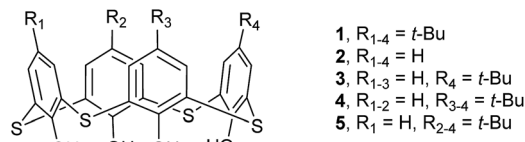
Fig. 2 Structures of compounds 1–5.
