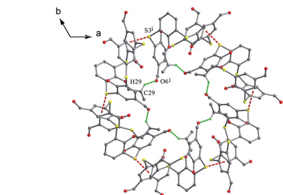
Fig. 100 A disc-like hexamer of 110 built by C-H \cdots O and S \cdots \pi interactions.
