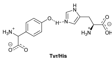
Fig. 1 Scheme of tyrosine/histidine pair in PS II.
