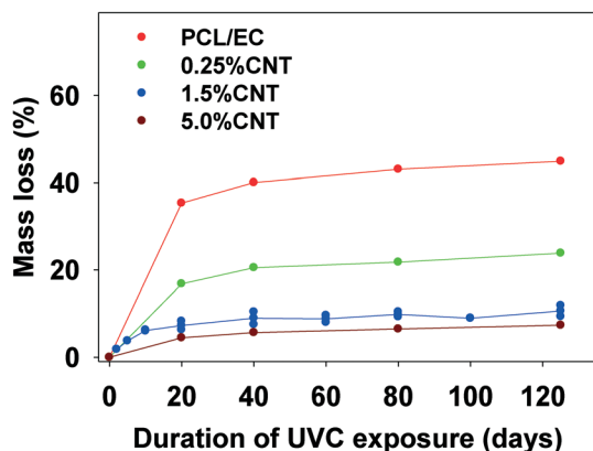
Fig. 2 Mass loss of SWCNT-PCL nanocomposites with varying SWCNT loading (% w/w) following incremental periods of irradiation with 254 nm light. The average initial mass of all samples used in the study is 31.0 mg ( \pm 2.3 mg).
