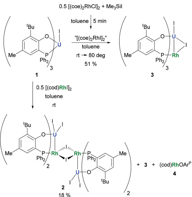
Scheme 1 Reactions of 1 with [(\text{cod})\text{RhI}]_2 and in situ generated [(\text{coe})_2\text{RhI}]_2 , respectively.
