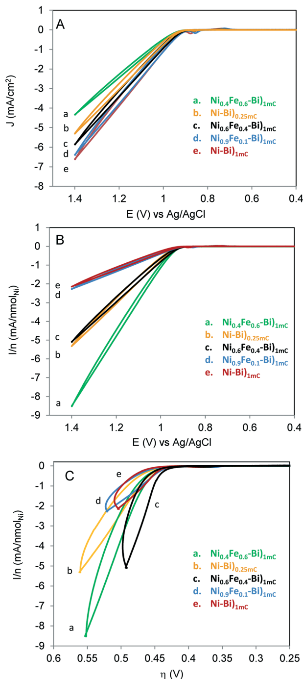
Fig. 7 Cyclic voltammograms (A), and the cyclic voltammograms plotted as current divided by nmol of Ni vs. potential (B) and current per nmol of Ni vs. overpotential \eta ( E - E_{eq}(O_2/H_2O) - iR ) (C) at anodically-conditioned Ni 0.4 Fe 0.6 -Bi) 1mC (a), Ni-Bi) 0.25mC (b) Ni 0.6 Fe 0.4 -Bi) 1mC (c), Ni 0.9 Fe 0.1 -Bi) 1mC (d), and Ni-Bi) 1mC (e). Scan rate is 10 mV s -1 . Electrolyte is 1 M KBI ~pH 9.16.
