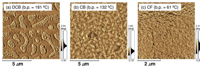
Fig. 10 AFM phase images of P3HT/PF12TBT blend films spin-coated from (a) DCB (b) CB, and (c) CF solutions of P3HT and PF12TBT (1 : 1 weight ratio), on glass substrates and annealed at 140 °C for 10 min.
