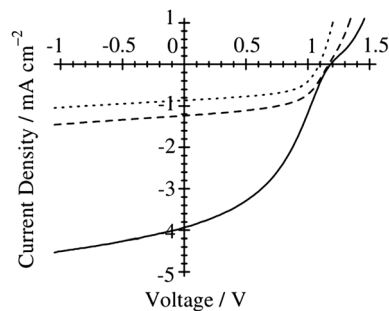
Fig. 9 J - V characteristics of P3HT/PF12TBT solar cells under AM 1.5G 100 \text{mW cm}^{-2} illumination. The devices were fabricated via spin-coating from DCB (dotted line), CB (dashed line), and CF (solid line) solutions of P3HT and PF12TBT (1 : 1 weight ratio) and annealed at 140 °C for 10 min. Adapted with permission from (ref. 41). Copyright 2011, American Chemical Society.
