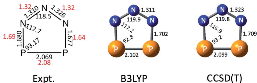
Fig. 2 Comparison of the X-ray structure of P_2N_3^- in [Na-kryptofix-221][ P_2N_3^- ] salt (major component in black, minor component in red) 27 with the calculated structures at B3LYP/aug-cc-pVTZ and CCSD(T)/aug-cc-pVTZ levels of theory. Bond distances are in angstroms (Å) and bond angles are in degrees (°).
