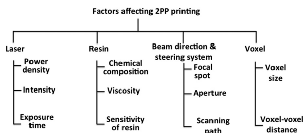
Fig. 15 Parameters affecting 2PP print process.
