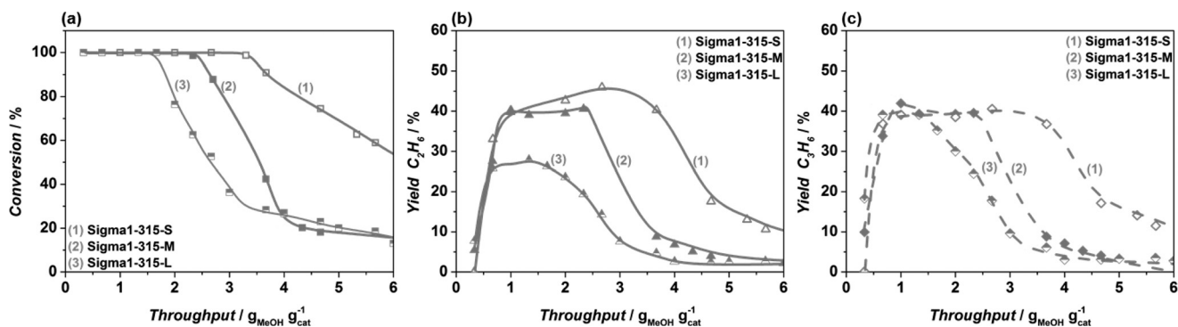
Fig. 7 Methanol conversion (a), yield of ethylene (b) and propylene at 450 °C, obtained in MTO reaction over Sigma1-315-S (□, ▲, ◆, ■), Sigma1-315-M (■, ▲, ◆, ■), Sigma1-315-L (◆, ▲, ■) zeolite at standard operation conditions.
