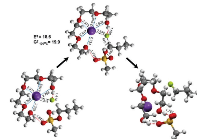
Fig. 7 Calculated structures of pre-reaction complexes, transition states and post-reaction complexes in the mechanism for the reaction [\text{K}^+\text{F}^- + \text{C}_3\text{H}_7\text{-OMs} \rightarrow \text{K}^+\text{OMs}^- + \text{C}_3\text{H}_7\text{-F}] in tetraEG. Energy and Gibbs free energy in \text{kcal mol}^{-1} and bond lengths in Å (MPW1K/6-31++G**).
