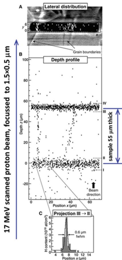
Fig. 2 Depth profiling H in polycrystalline diamond with high lateral resolution. From Fig. 3 of Reichart et al. , Science , 2004. 32 Reprinted with permission from AAAS.
