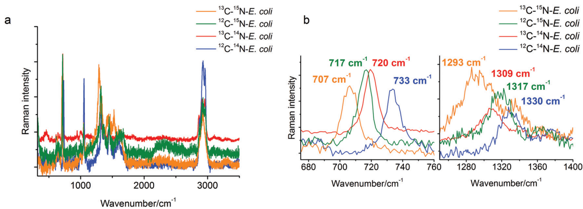
Fig. 1 (a) Overlay of the SERS spectra of single E. coli cells grown with either ^{12}\text{C} -glucose/ ^{14}\text{N} -ammonium chloride, ^{13}\text{C} -glucose/ ^{14}\text{N} -ammonium chloride, ^{12}\text{C} -glucose/ ^{15}\text{N} -ammonium chloride or ^{13}\text{C} -glucose/ ^{15}\text{N} -ammonium chloride; (b) a red-shift of the SERS marker band at 733\text{ cm}^{-1} for ^{12}\text{C} - ^{14}\text{N} - E. coli to 720\text{ cm}^{-1} for ^{13}\text{C} - ^{14}\text{N} - E. coli , to 717\text{ cm}^{-1} for ^{12}\text{C} - ^{15}\text{N} - E. coli , and to 707\text{ cm}^{-1} for ^{13}\text{C} - ^{15}\text{N} - E. coli could be found in the SERS spectra. The band at 1330\text{ cm}^{-1} of ^{12}\text{C} - ^{14}\text{N} - E. coli is red-shifted to 1317\text{ cm}^{-1} for ^{12}\text{C} - ^{15}\text{N} - E. coli , to 1309\text{ cm}^{-1} for ^{13}\text{C} - ^{14}\text{N} - E. coli , and to 1293\text{ cm}^{-1} for ^{13}\text{C} - ^{15}\text{N} - E. coli .
