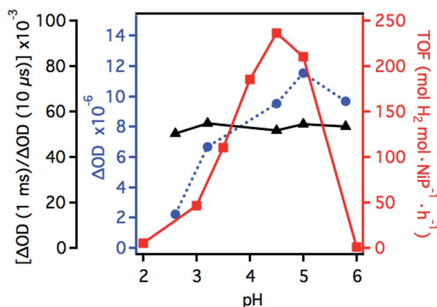
Fig. 4 \text{TOF}_{\text{NiP}}(\text{H}_2) of a homogeneous AA (0.1 M) aqueous solution at different pH values, containing RuP (0.3 \mu\text{M} , 133 \mu\text{M} ) and NiP (0.1 \mu\text{M} , 44 \mu\text{M} ; red squares). Transient absorption signal amplitudes of the NiP bleach at 1 ms (absolute values, blue circles) and transient absorption amplitude ratios of NiP at 1 ms and RuP − at 10 \mu\text{s} (black triangles).
