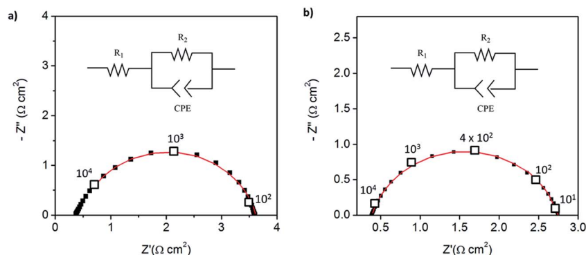
Fig. 6 Symmetric cell impedance measurements of 30 wt% Pt-CNT based electrodes prepared by (a) strategy 1 (see Scheme 2) in which Pt-CNT bearing and CDP bearing solutions were electro-sprayed sequentially, and (b) strategy 2 in which a single Pt-CNT and CDP bearing solution was sprayed. In (a), the Pt loading and utilization are 4.2 \times 10^{-3} \text{ mg cm}^{-2} Pt and 64 \text{ S mg}^{-1} , respectively, whereas in (b) they are 5.1 \times 10^{-3} \text{ mg cm}^{-2} Pt and 86 \text{ S mg}^{-1} . Measurements are performed at 240^\circ \text{C} in a dynamic atmosphere of 0.4 \text{ atm H}_2\text{O} and balance \text{H}_2 supplied at a gas velocity of 6 \text{ cm min}^{-1} and spectra are taken after 4 hours (insets: equivalent circuit used for fitting).
