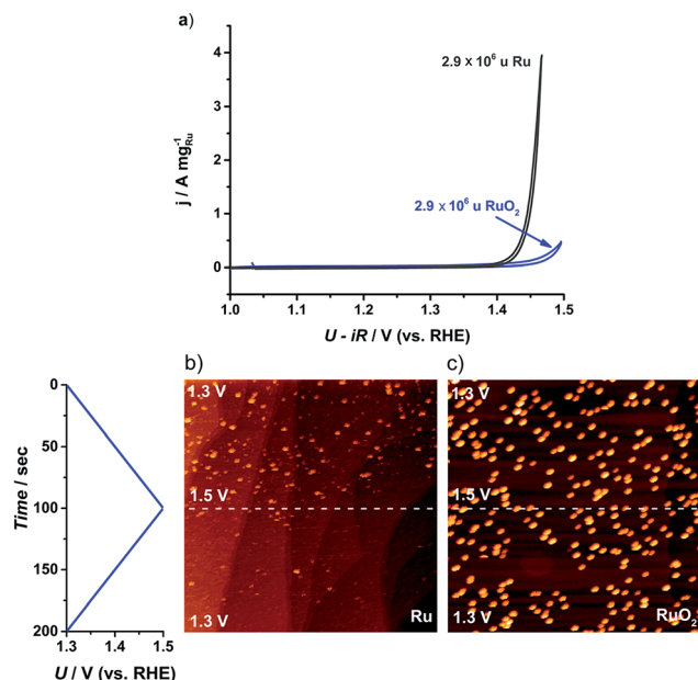
Fig. 5 (a) Cyclic voltammogram (CV) for the first cycle of the as-deposited Ru and thermally oxidized \text{RuO}_2 2.9 \times 10^6 u nanoparticles on GC. CV recorded in \text{N}_2 saturated 0.05 \text{ M H}_2\text{SO}_4 between 1.0 and 1.5 V (vs. RHE) at 20 \text{ mV s}^{-1} and 1600 rpm. (b) and (c) Potentiodynamic STM images of Ru dissolution in Ar-saturated 0.05 \text{ M H}_2\text{SO}_4 solution. The potential was scanned between 1.3 and 1.5 V (vs. RHE) at 2 \text{ mV s}^{-1} : (b) 0.001 monolayer of as-deposited 0.1 \times 10^6 u Ru nanoparticles, (520 \text{ nm})^2 , U_B = -299 \text{ mV} , I_T = 1 \text{ nA} ; (c) 0.001 monolayer of thermally treated 0.1 \times 10^6 u \text{RuO}_2 nanoparticles, (516 \text{ nm})^2 , U_B = -245 \text{ mV} , I_T = 1 \text{ nA} .
