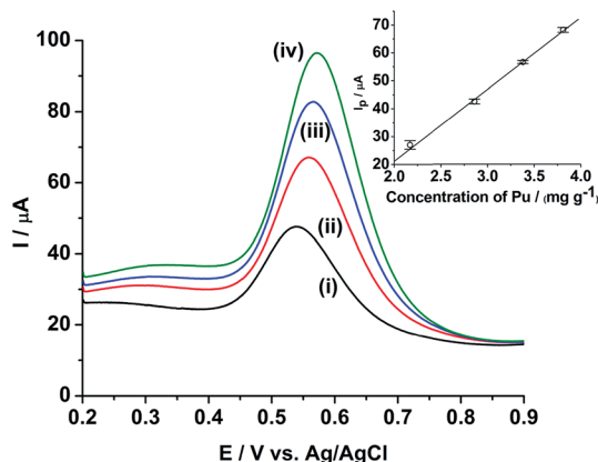
Fig. 5 ASWVs of (i) 2.17, (ii) 2.86, (iii) 3.38 and (iv) 3.81 mg g -1 of Pu in 1 M H 2 SO 4 on rGO/GC. Square wave amplitude = 25 mV; square wave frequency = 20 Hz; step potential increment = 1 mV; hold time at initial potential = 10 s. Inset shows the sensitivity plot for the same. The vertical bars shown in the inset represent the standard deviation ( \sigma ) of I_p obtained from ten replicate measurements for each concentration of Pu.
