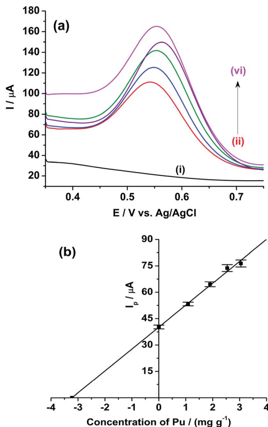
Fig. 10 ASWVs of the (i) blank 1 M H_2SO_4 (ii) of (U, Pu)C FBTR sample in 1 M H_2SO_4 and standard addition of (iii) 1.088 mg\ g^{-1} , (iv) 1.904 mg\ g^{-1} , (v) 2.539 mg\ g^{-1} and (vi) 3.047 mg\ g^{-1} of standard plutonium solution into the sample solution. Square wave amplitude = 25 mV; square wave frequency = 20 Hz; step potential increment = 1 mV; standby time at 0.35 V is 10 s. The error bars represent the standard deviation for ten repetitive measurements.
