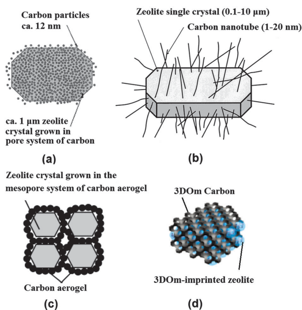
Fig. 2 Schematic diagram showing mesoporous zeolite templated by different forms of carbon materials: (a) carbon nanoparticles, (b) carbon nanotubes, (c) carbon aerogel and (d) 3D ordered mesoporous (3DOM) carbon. (Adapted from ref. 29, 34, 38 and 53.)
