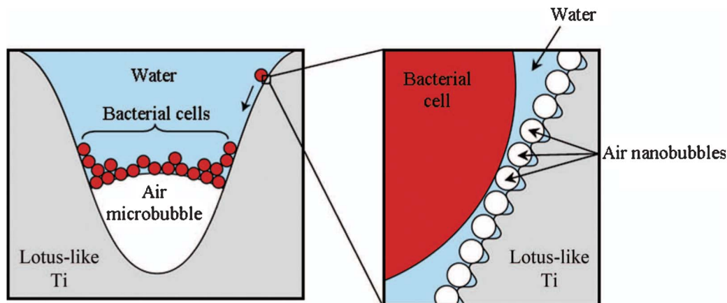
Fig. 13 Proposed mechanism by which bacterial cells accumulate at the tri-phase interface on immersed superhydrophobic Ti surfaces. Reprinted by kind permission of Taylor & Francis Ltd, from Air-directed attachment of coccoid bacteria to the surface of superhydrophobic lotus-like titanium, V. K. Truong, H. K. Webb, E. Fadeeva, B. N. Chichkov, A. H. F. Wu, R. Lamb, J. Y. Wang, R. J. Crawford and E. P. Ivanova, Biofouling: the Journal of Bioadhesion and Biofilm Research , 2012, 28 , 539–550.
