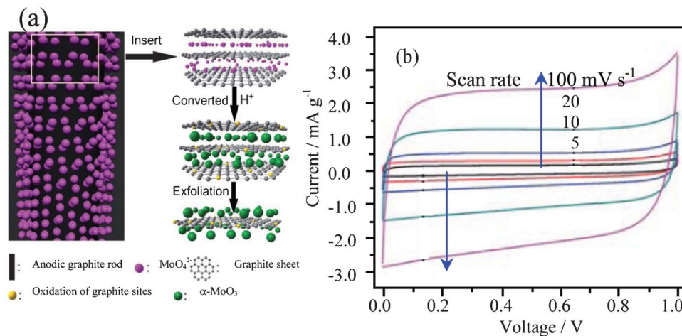
Fig. 11 (a) Illustration of the formation of the composite of \alpha - \text{MoO}_3 -decorated graphene sheets by electrolytic exfoliation from graphite with the assistance of molybdate and (b) CV curves of the composite in 6 \text{ mol l}^{-1} KOH (modified from ref. 49a).
