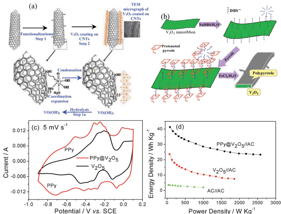
Fig. 3 Schematic illustration for the synthesis of (a) \text{V}_2\text{O}_5 @CNTs (modified from ref. 37a) and (b) \text{PPy} @ \text{V}_2\text{O}_5 , (c) CV curves of \text{V}_2\text{O}_5 and \text{PPy} @ \text{V}_2\text{O}_5 in 0.5 \text{ mol l}^{-1} \text{ K}_2\text{SO}_4 solution, and (d) Ragone plots of the ASC of \text{V}_2\text{O}_5 //AC and \text{PPy} @ \text{V}_2\text{O}_5 //AC using 0.5 \text{ mol l}^{-1} \text{ K}_2\text{SO}_4 solution as the electrolyte (The capacitance and energy densities were calculated based on the total mass of two active electrode materials) (modified from ref. 6b).
