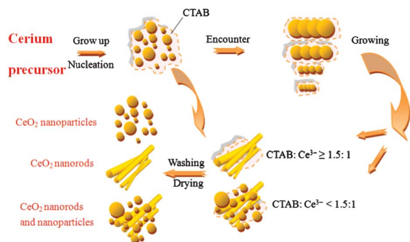
Fig. 4 Schematic diagram of the proposed mechanism for the formation of the CeO 2 nanostructures at room temperature.
